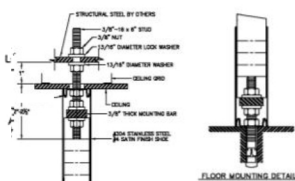
FLOOR MOUNTING DETAIL
