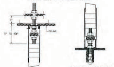
FLOOR ANCHOR DETAIL
